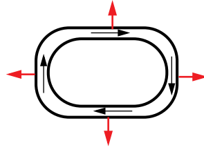
Fig.7 Magnetic forces between oppositely oriented circuit elements.
