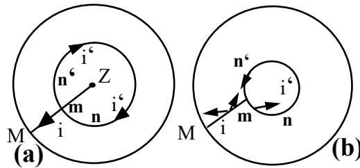
Fig.9 (a) The arrows indicate the tangential microscopic current i' of the magnet and the radial macroscopic current i flowing outside the magnet. (b) The arrows indicate the attractive forces of action and reaction acting between i' in the portion m-n' and i , and the repulsive forces of action and reaction between i' in the portion nm and i .
