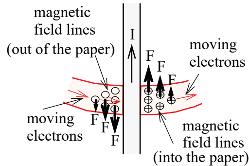
Fig.5 Magnetic forces on a current-carrying solenoid due to the magnetic field of a traversing external current.
