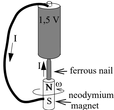
Fig.1 The "simplest" motor.
