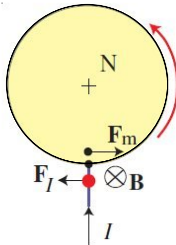
Fig.4 Top view of the magnet indicating the action and reaction forces 6 (see text).
