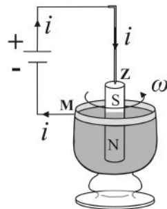
Fig.6 (a) A schematic representation of Ampère's motor.
