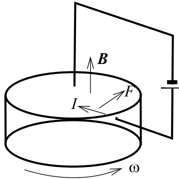
Fig.2 Schematic representation of magnet and circuit together with an indication of the magnetic force F .
